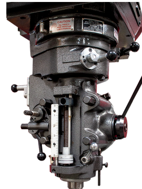
EXAMPLE OF MVM HEAD
