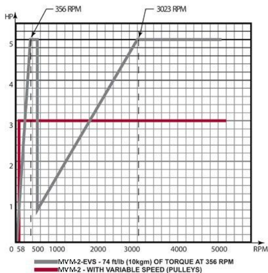
POWER &amp; SPEED DIAGRAM
