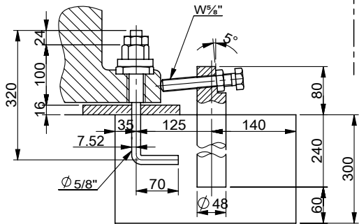
Y-Y view
