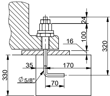
X-X view
