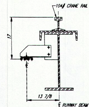
© INSUL-8 "SAFE-LEC 2" (400 AMP) RUNWAY CONDUCTOR SYSTEM BY WHITING CORPORATION. SEE DRG. T-74259
