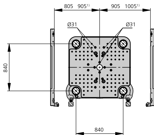
Moving mould mounting platen | B
