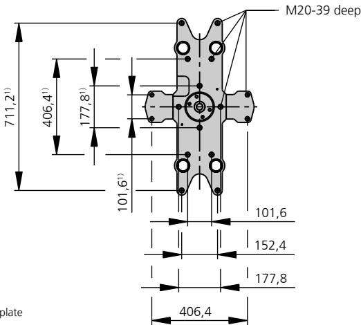
Ejector plate | D
