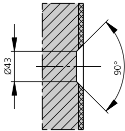
Bore in mould (if required) | Y
