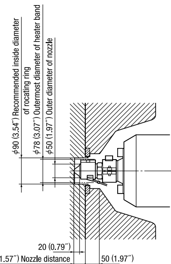
Nozzle section
