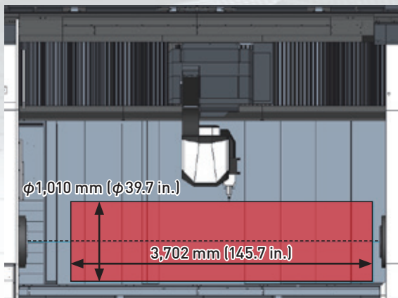
When B-axis is at 90°: \phi 1,010 \times 3,702 mm ( \phi 39.7 \times 145.7 in.)
