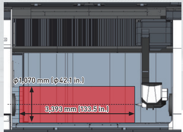
When B-axis is at 0°: \phi 1,070 \times 3,393 mm ( \phi 42.1 \times 133.5 in.)
