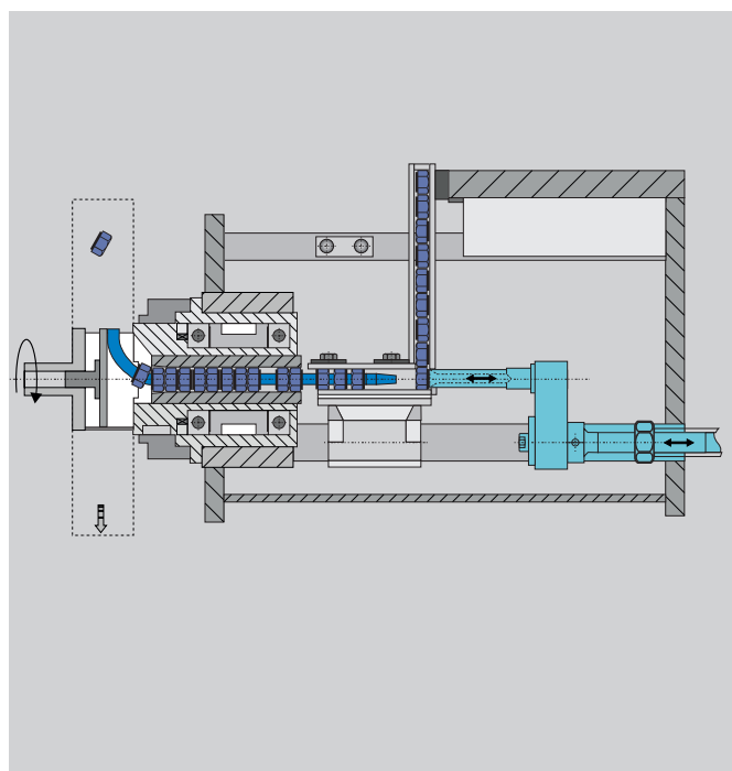
▲ Tool arrangement
