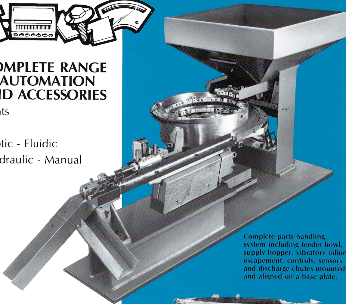
Standard Screw Feeder
