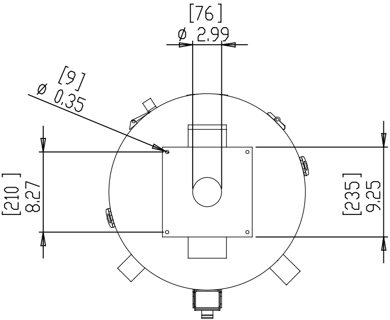
MOUNTING PLATE DETAIL
