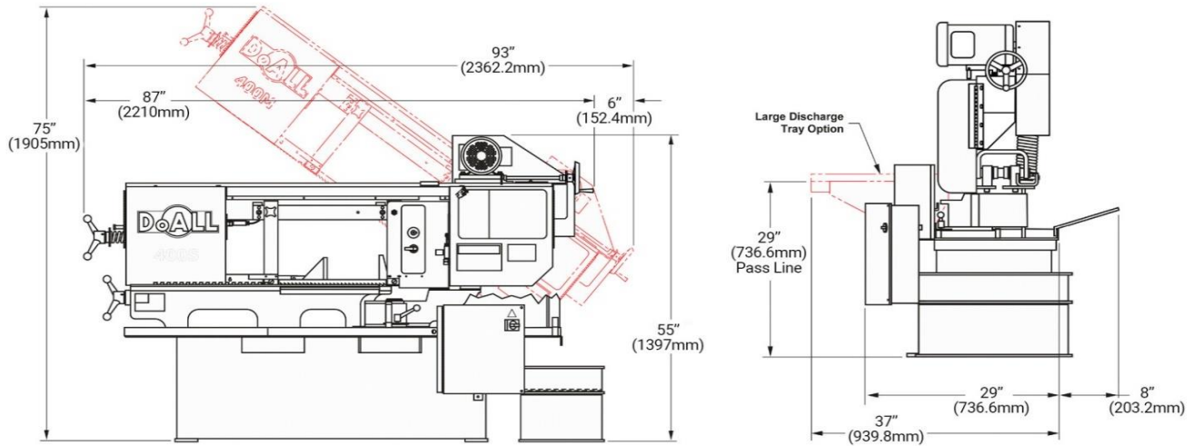
Dimensional Drawings of 400-S
