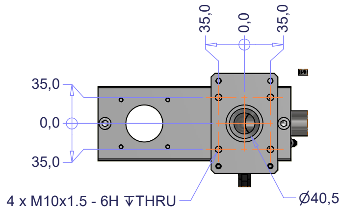
HOPPER CONNECTION
