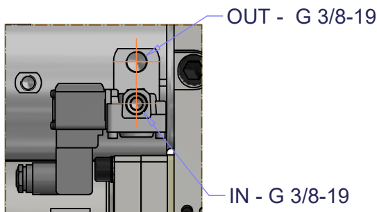
VIEW FROM C COOLING CONNECTION
