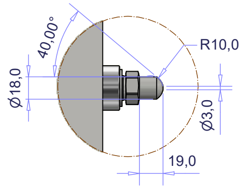
DETAIL B - OPEN NOZZLE
