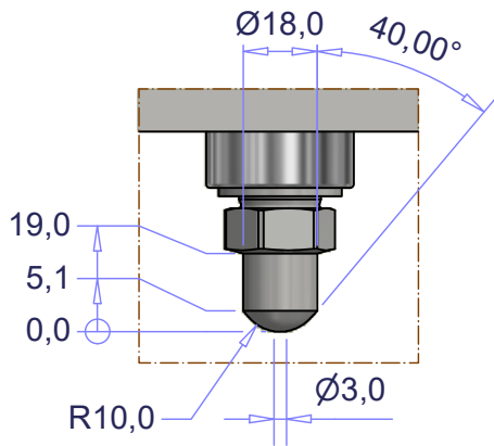
VIEW B OPEN NOZZLE
