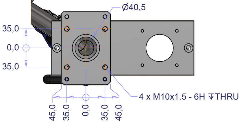
HOPPER CONNECTION
