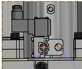
VIEW FROM D COOLING CONNECTION
