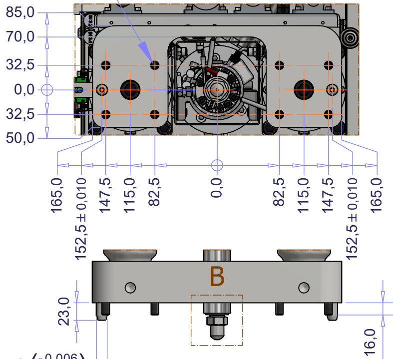
VIEW B OPEN NOZZLE
