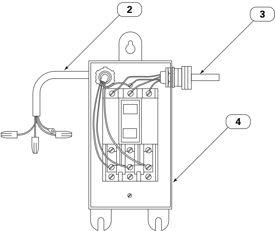
Manual Starter Assembly, 3 Phase (Model 81, 85 Single Phase Shown)
