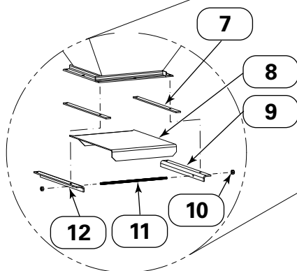
55-Gallon Drum Cover with Slide Gate Model 90 Only
