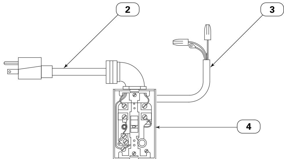
Manual Starter Assembly, Models 54-75 Single Phase
