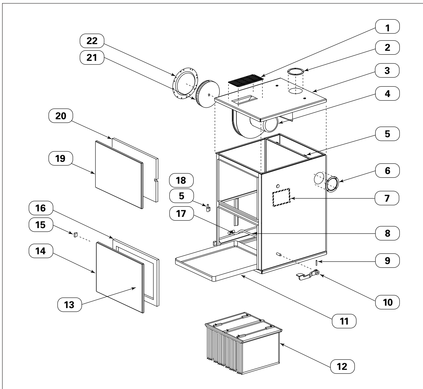
Cabinet 54-84 Dust Collector
