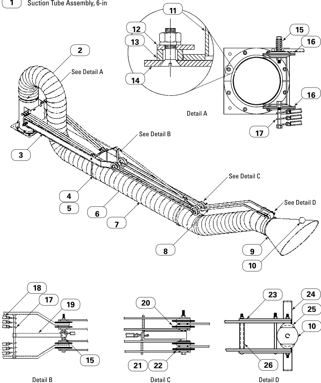
6-in Suction Tube Assembly
