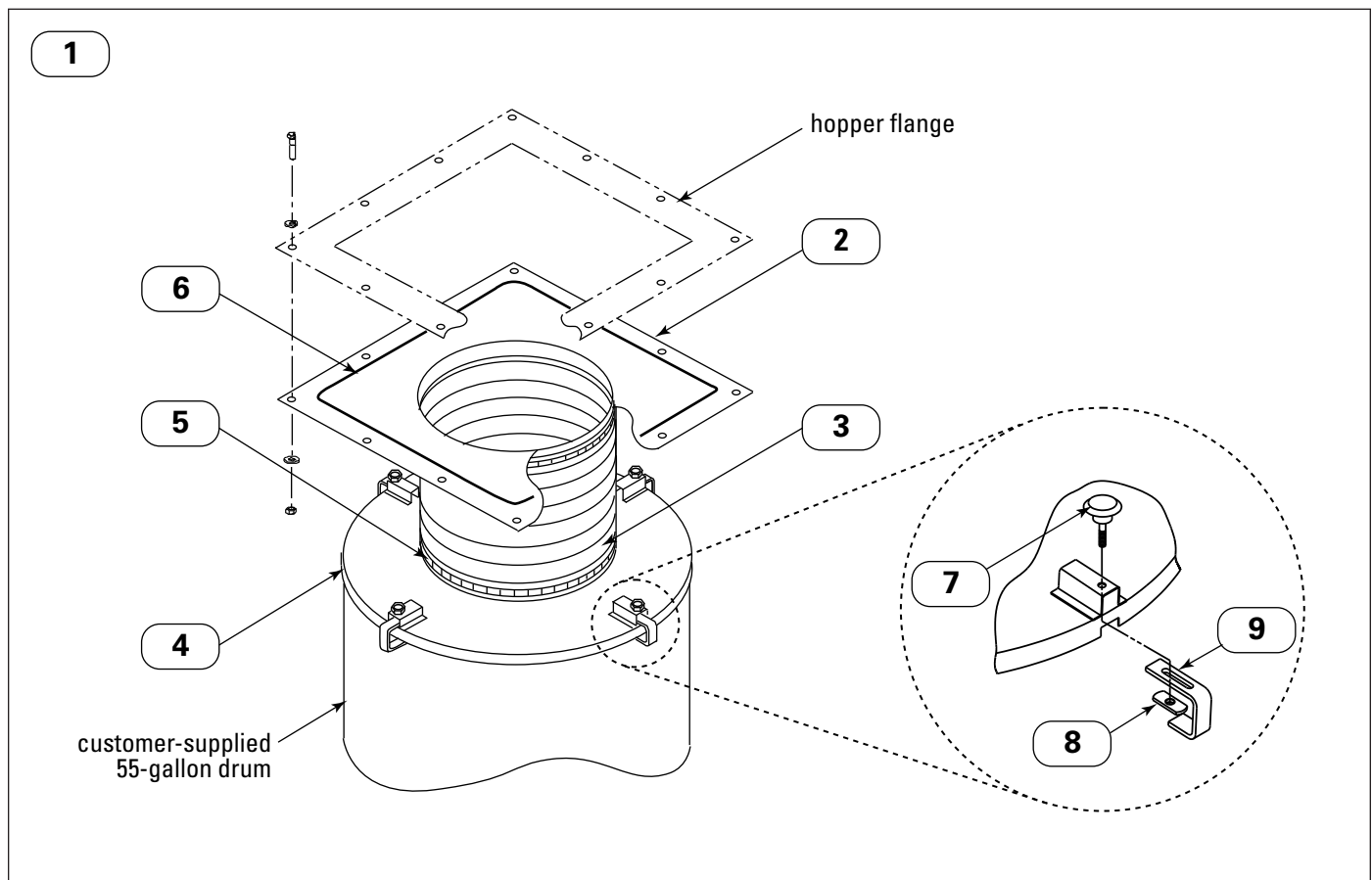
55-Gallon Drum Cover Assembly
