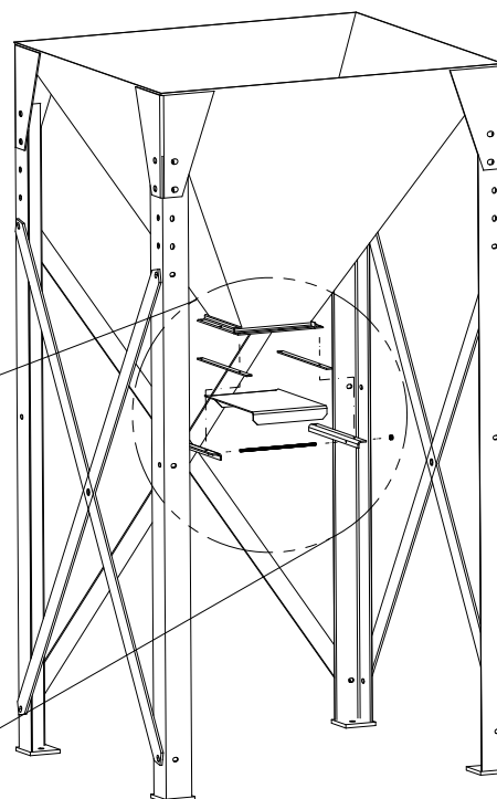
Cabinet 90 Hopper Pack Slide Gate Only Without Drum Cover
