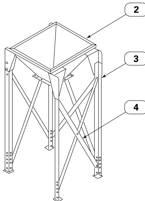
55-Gallon Hopper Assembly
