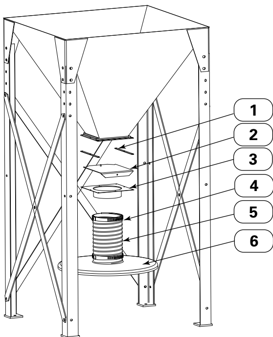
Cabinet 90 Hopper Pack with Drum Cover With or Without Slide Gate
