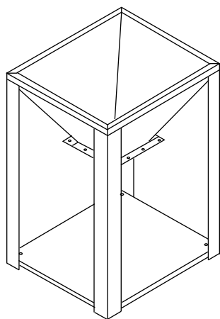
5-Gallon Hopper Assembly
