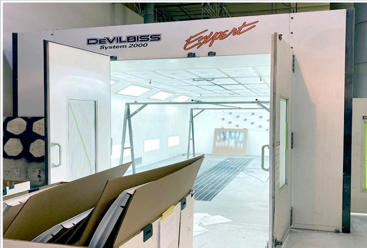
DEVILBISS SYSTEM Downdraft Pressurized Spray Booth
