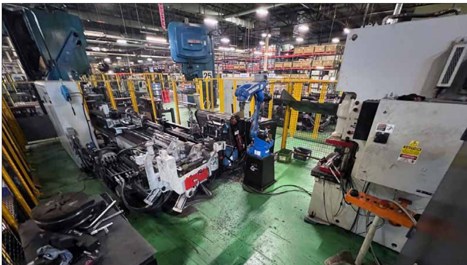
Complete Robotic Press Cell - STAMTEC OCP-45 45-Ton Press, with Yaskawa GP12 Robot, YRC1000 Controller, UTE Tube Loader & Full Safety Enclosure
